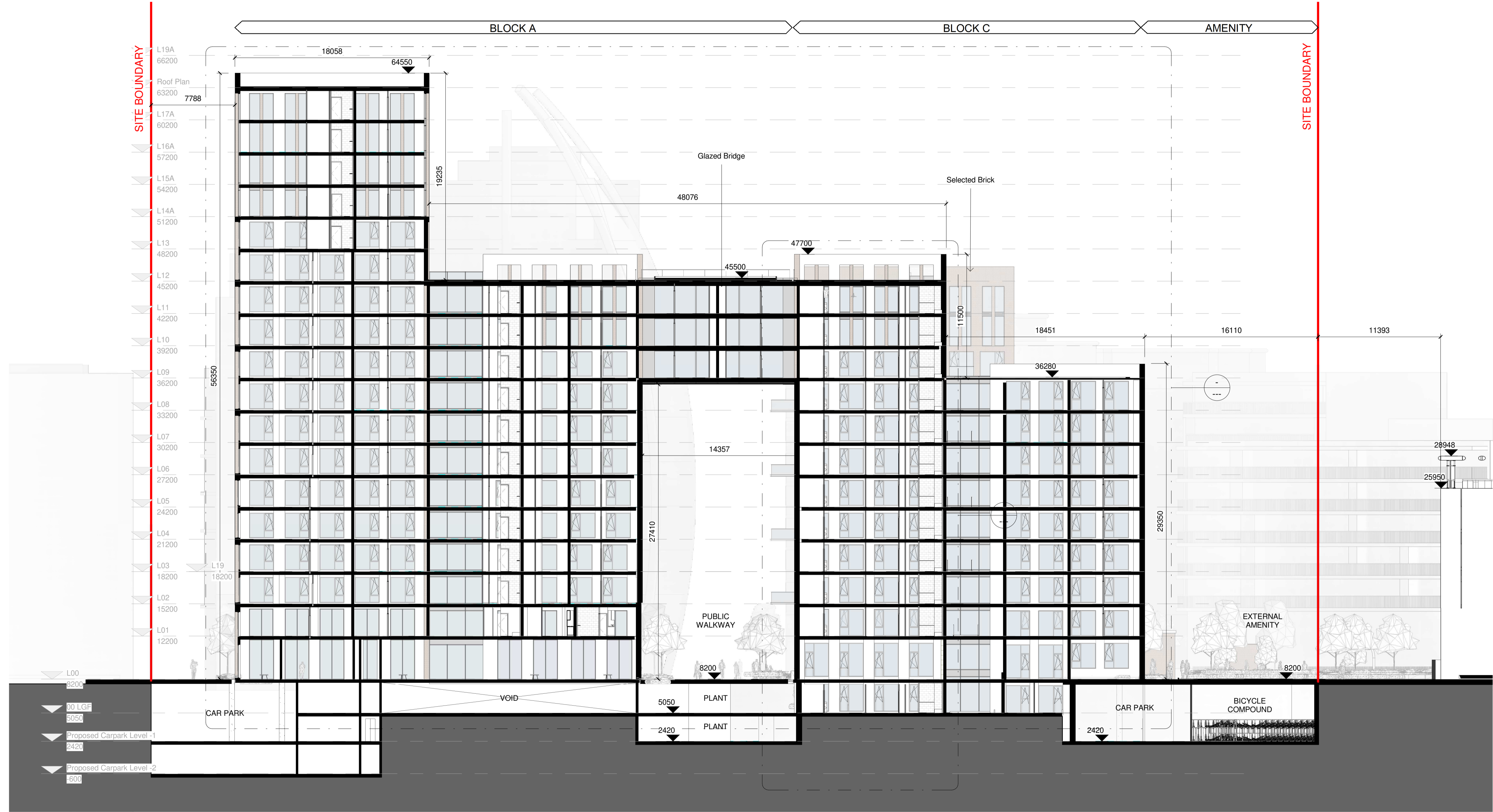
Proposed Section 01 1:200
